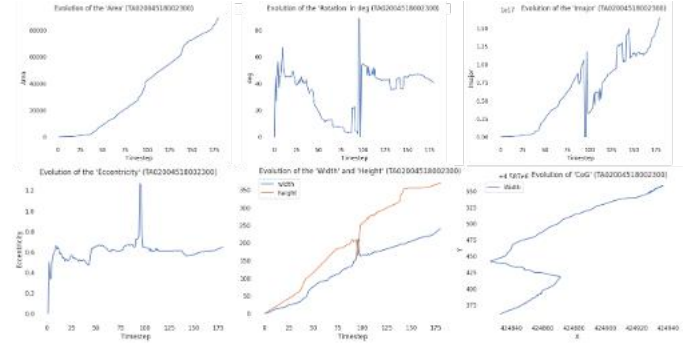
Figure 4. Illustrates the evolution of the six features: “Area,” “Rotation,” “Major,” “Eccentricity,” “Width,” “Height,” and “Center of Gravity of the contour” for each timestep.
